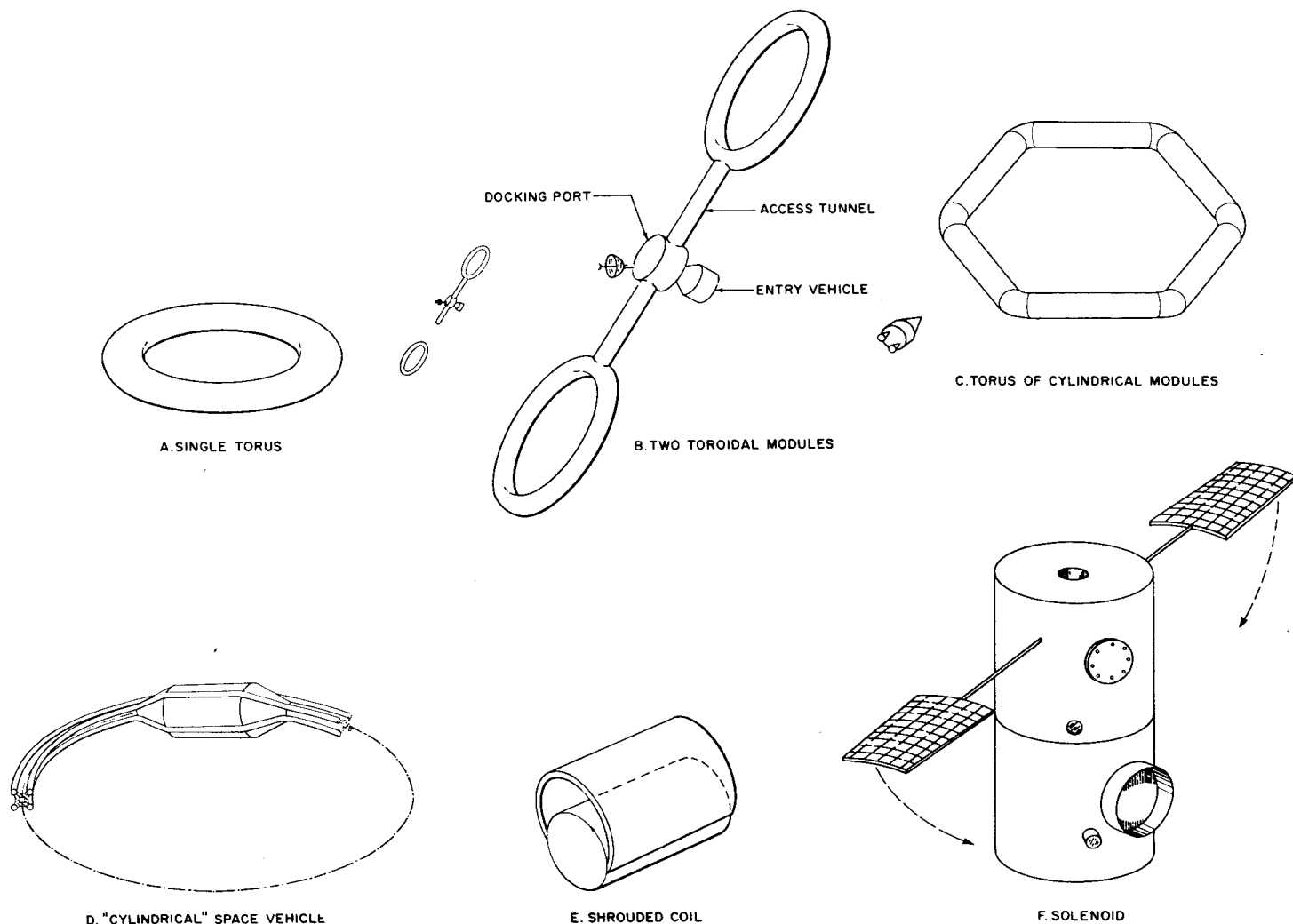
Fig. 5 Some possible configurations of spacecraft that utilize the plasma radiation shield concept.
