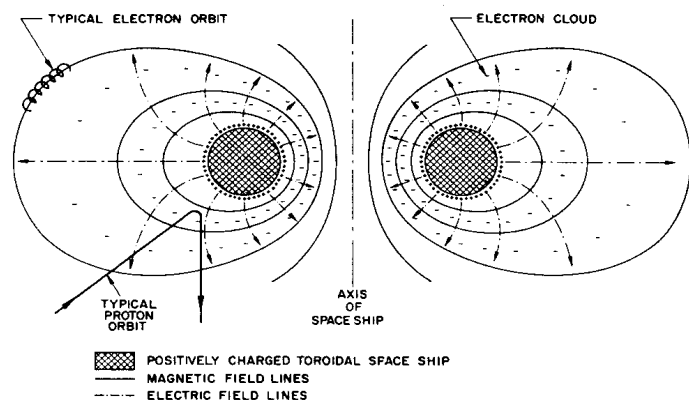
Fig. 3 Electric and magnetic field lines around a typical shield. The principal electron motion is an azimuthal drift around the axis of symmetry. The electrons may also have lesser motions along the magnetic field lines and around them in the manner shown.
