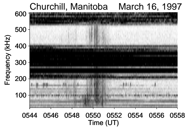
Figure 2. A raw spectrogram recorded by the swept frequency receiver during a time when auroral hiss occurs at frequencies from 30 kHz to above 500 kHz. Alternate sweeps are dark or light, showing that the waves are elliptically polarized. Careful inspection reveals that they are right-hand polarized, as expected on theoretical grounds and on the basis of previous measurements.
