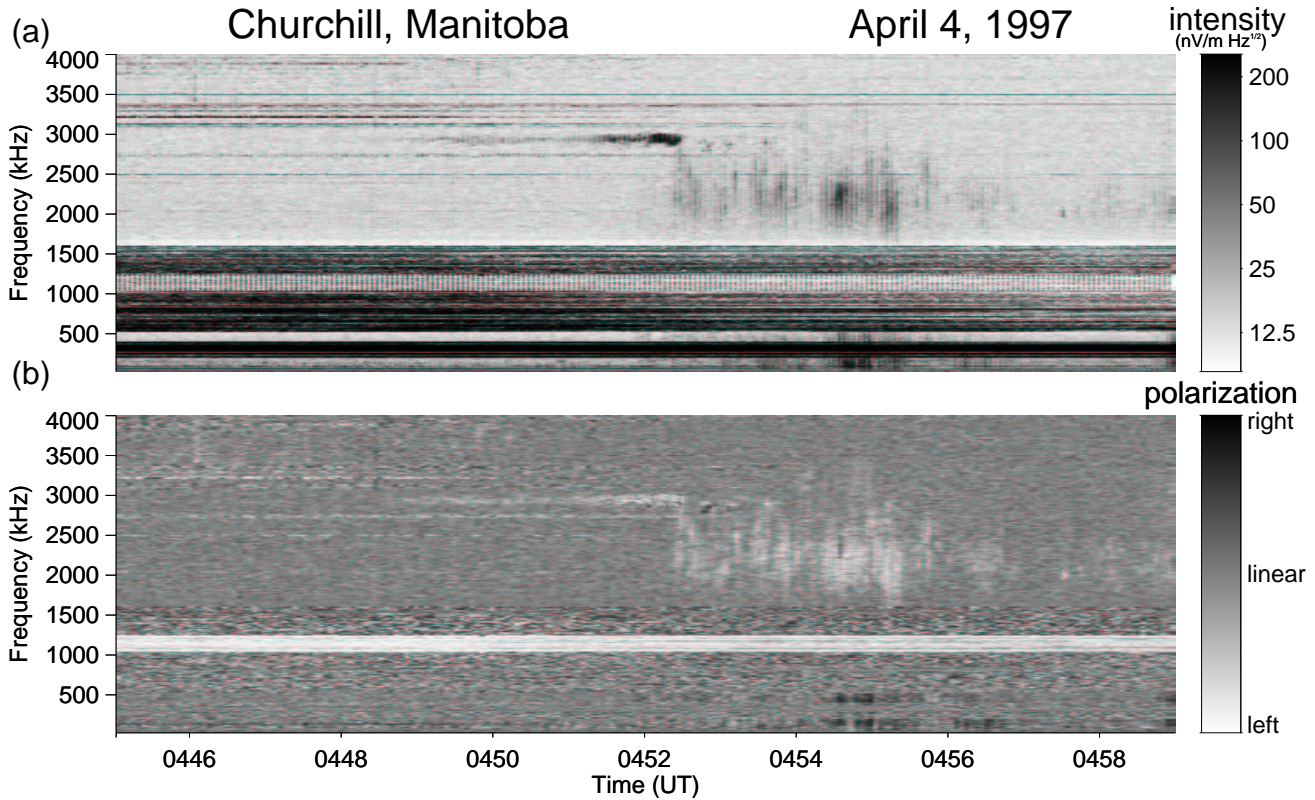
Figure 3. (a) Raw receiver output showing the three distinct types of emissions: auroral hiss, auroral roar, and MF-burst. The banded appearance of all three implies that they are elliptically polarized. (b) Polarization of emissions showing that auroral hiss is right-hand polarized, while MF-burst, auroral roar, and the calibration signal at 1.0–1.25 MHz are left-hand polarized.
