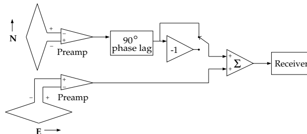
Figure 1. Schematic of polarization detection electronics. Phase shifting is represented as a 90^\circ lag of the signal in the N-S antenna loop. In reality, the phases of both signals are shifted to produce the 90^\circ lag.
