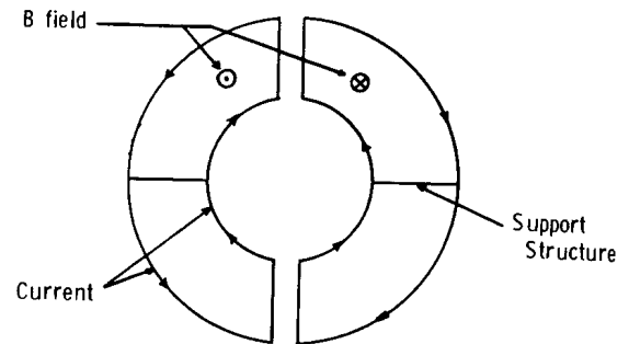
Fig. 2 Simplified sketch of hybrid torus magnetic field configuration.
