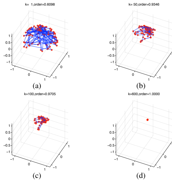
Fig. 2. Convergence to aligned state for a 3-D swarm of n = 100 agents.
