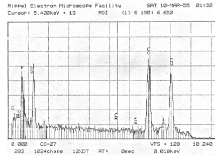
Fig. 2. EDS for a Co-MgF 2 TEM sample showing elemental spectral peaks.
