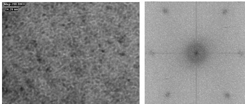
Fig. 1. TEM image (a) with associated FFT (b) for particle size determination. Inside edge of first circular region in FFT multiplied by 82% yields particle size. Shown above is a 41% cobalt sample deposited at 150°C.
