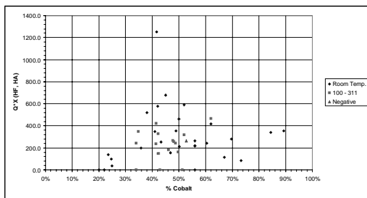
Fig. 4. Q\chi product versus volume percentage cobalt. Measured in the hard-axis direction with an applied field of \pm 1000 \text{ Oe} .
