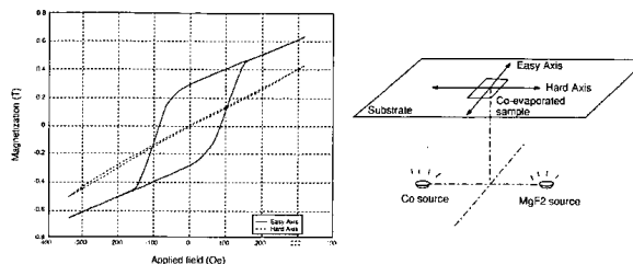
Fig. 1. (a) (left) Easy-axis and hard-axis M-H loops of a film deposited with no magnetic field applied. The anisotropy is found to be determined by the angles of evaporative deposition, as shown in (b)(right).
